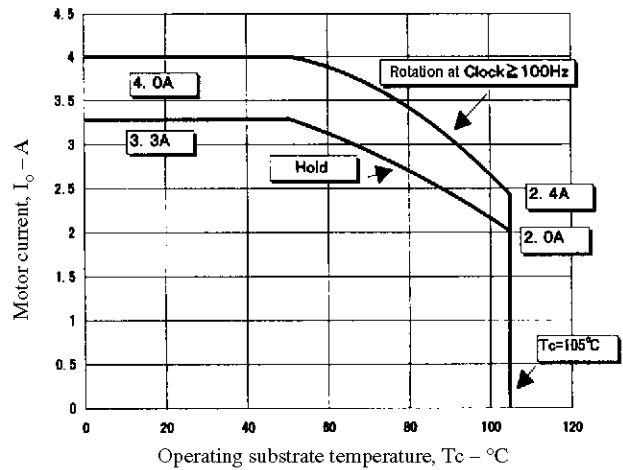
Figure 5. I_o - T_c
