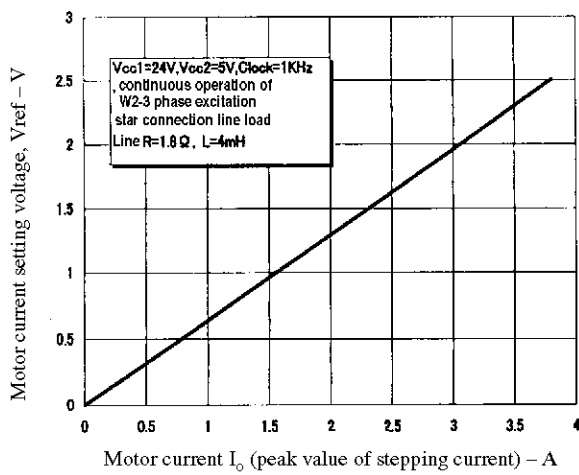
Figure 4. V_{ref} - I_o
