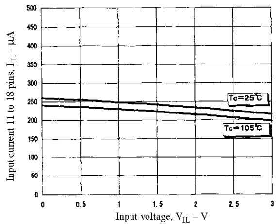
Figure 11. I_{IL} - V_{IL}
