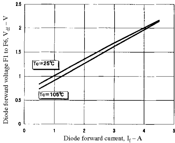
Figure 10. V_{df} - I_f
