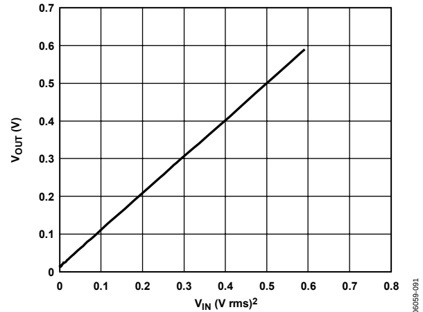
Figure 20. ADL5391 Used as Square Law Detector DC Output vs. Square of Input
