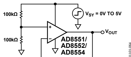
Figure 64. AD855x Test Circuit for Turn-On Time
