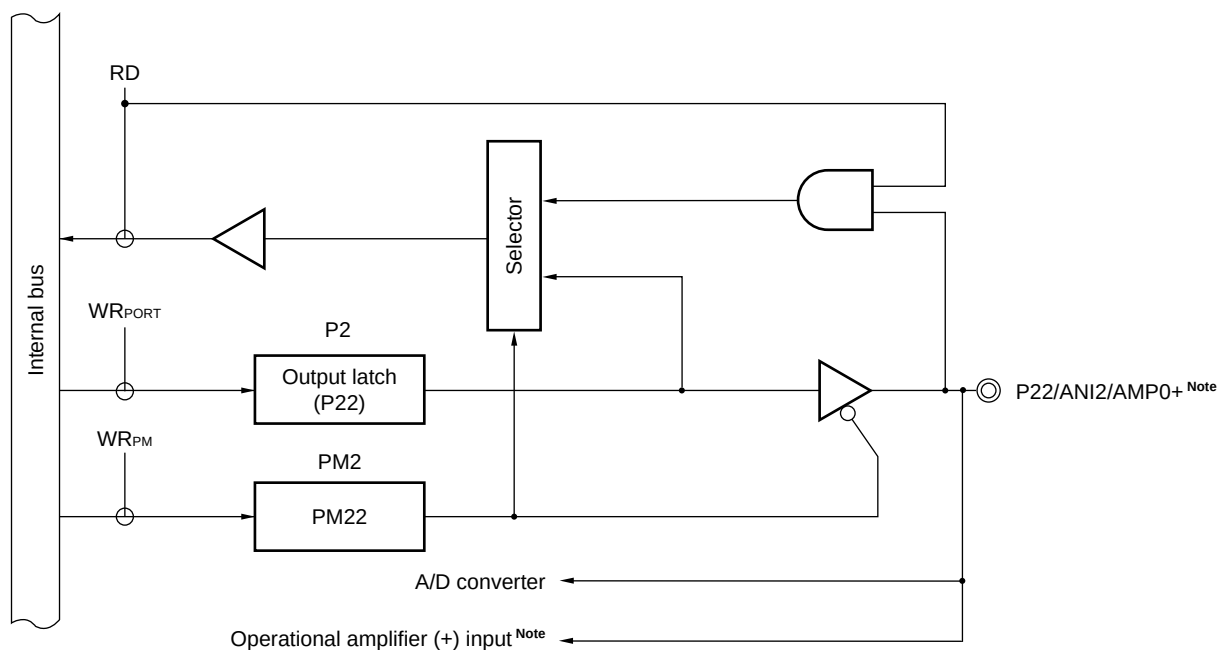
Figure 4-6. Block Diagram of P22
