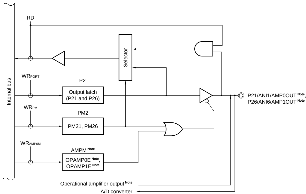
Figure 4-2. Block Diagram of P21 and P25
