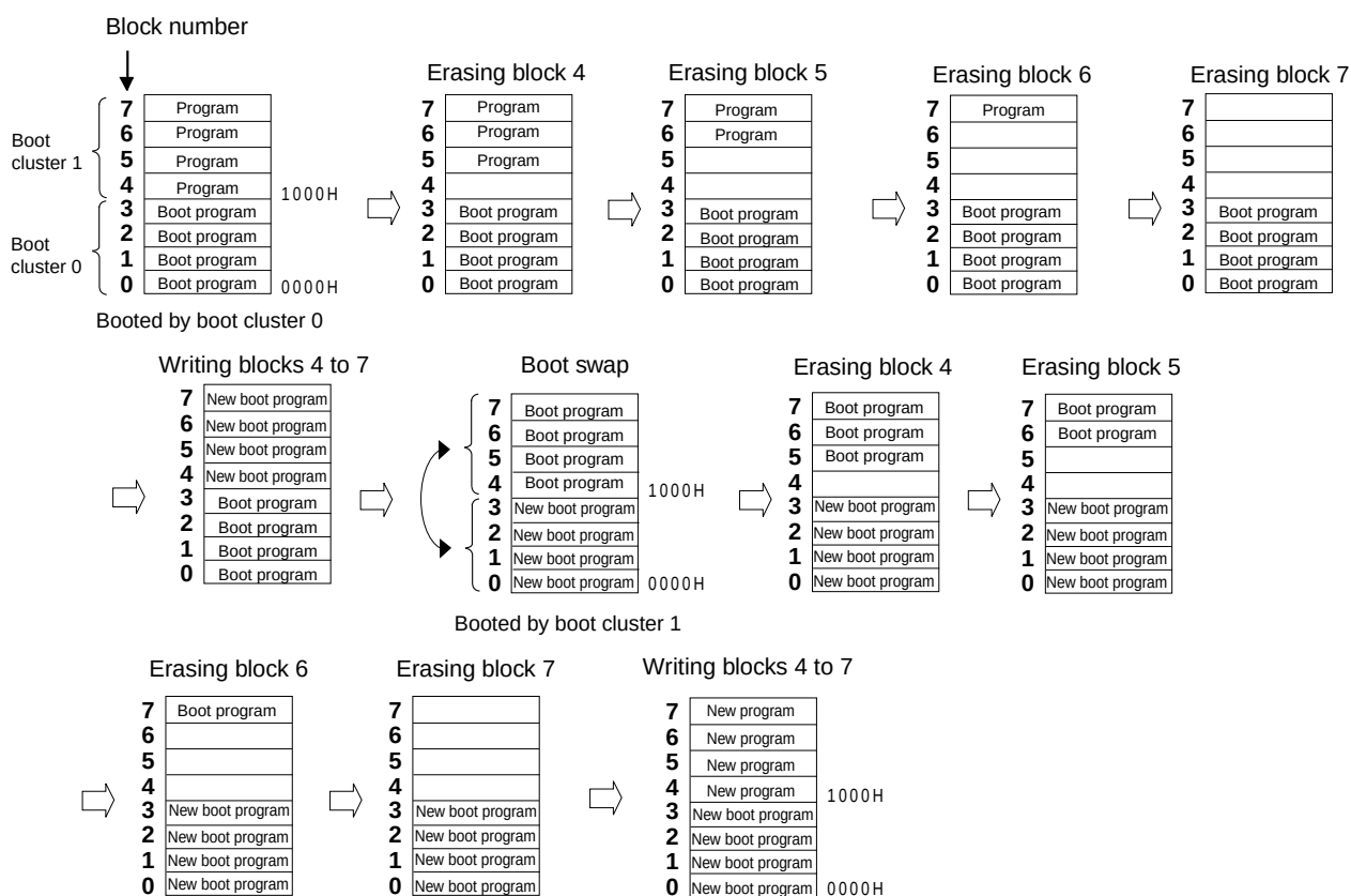
Figure 21-11. Example of Executing Boot Swapping
