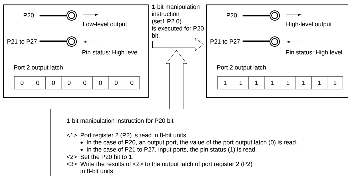
Figure 4-28 1-Bit Manipulation Instruction (P20)
