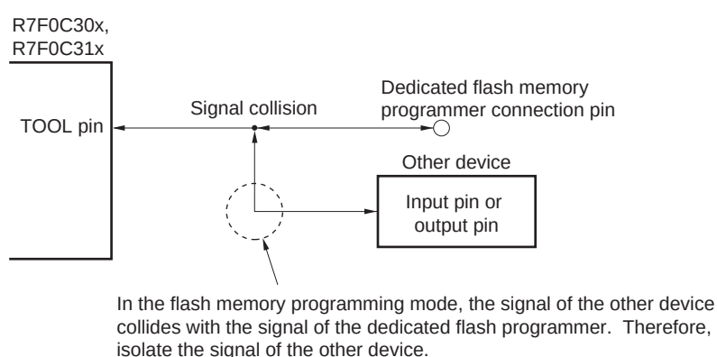
Figure 21-3. Signal Collision (TOOL Pin)
