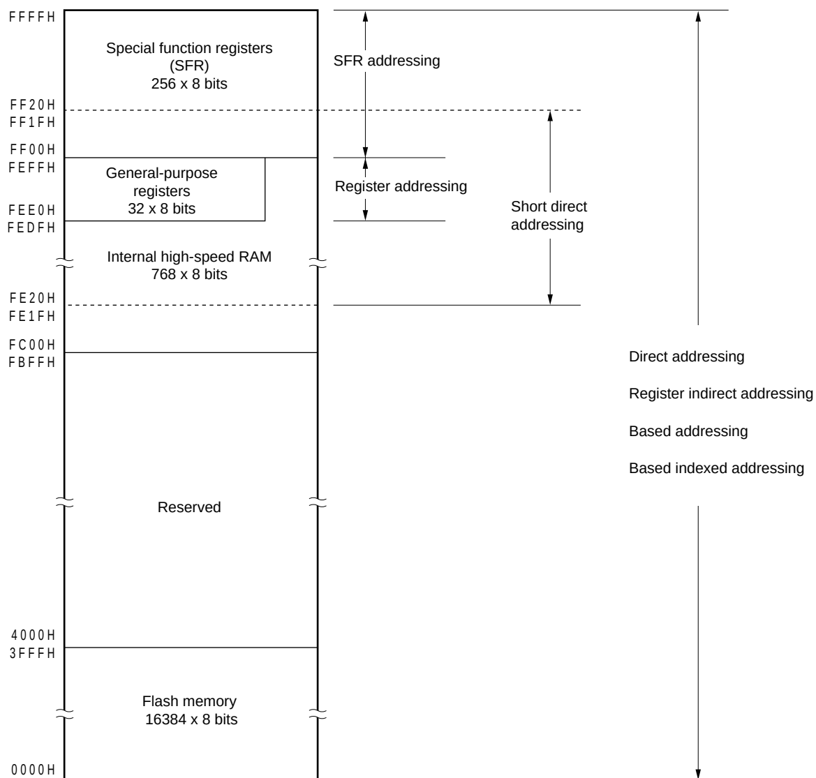
Figure 3-6. Correspondence Between Data Memory and Addressing (R7F0C302x, R7F0C305x, R7F0C308x, R7F0C311x)
