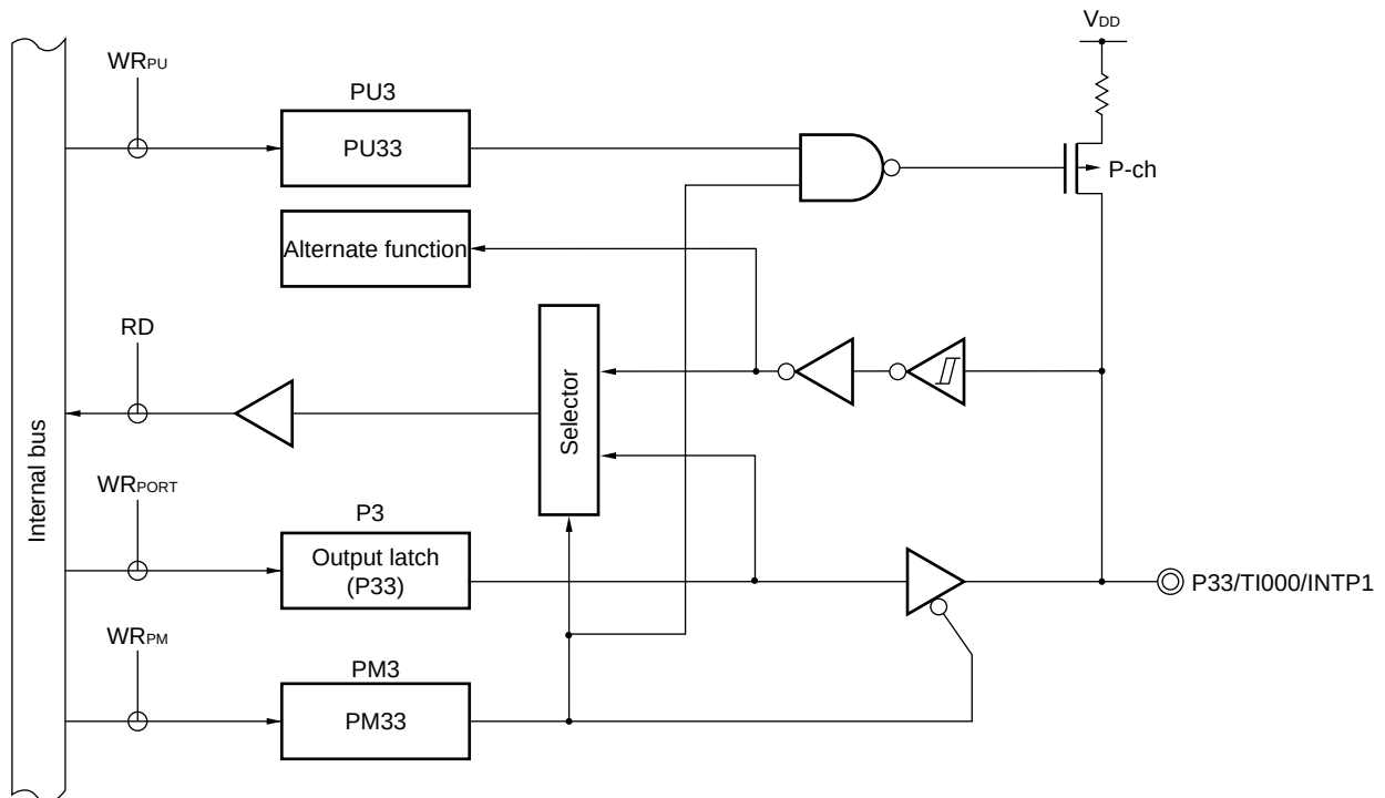
Figure 4-14. Block Diagram of P33
