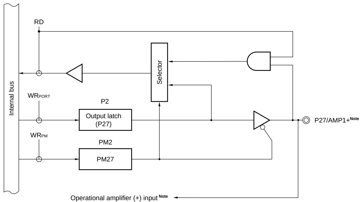
Figure 4-10. Block Diagram of P27
