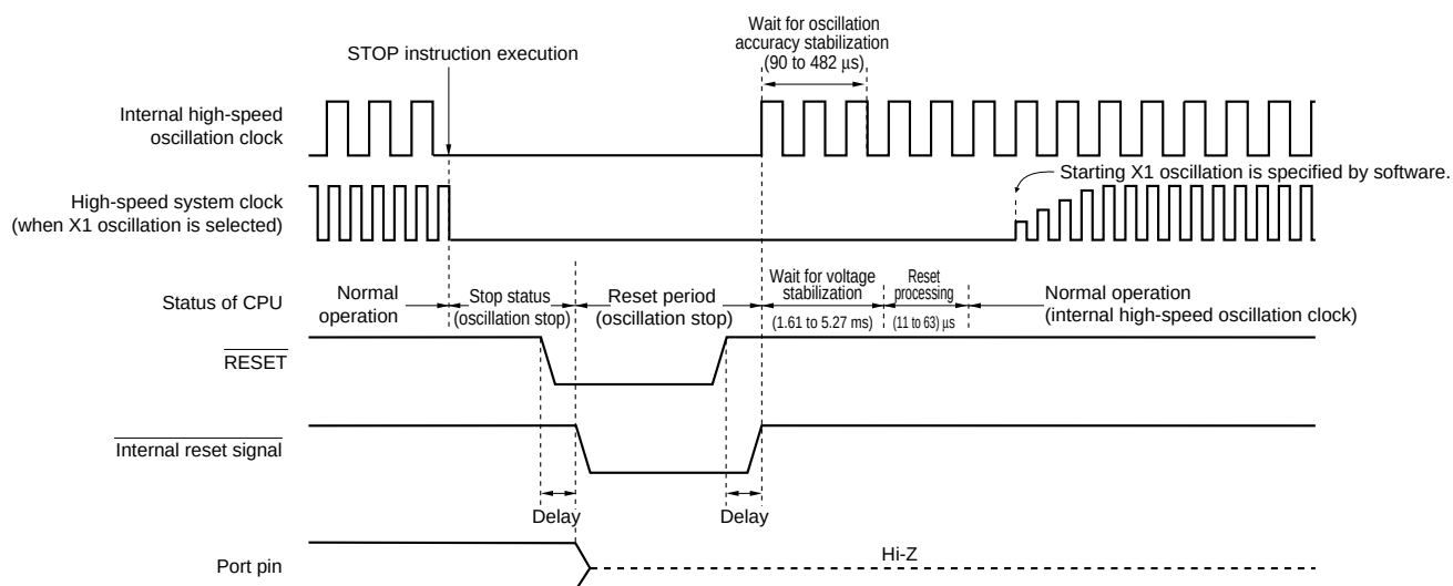
Figure 16-4. Timing of Reset in STOP Mode by \overline{\text{RESET}} Input
