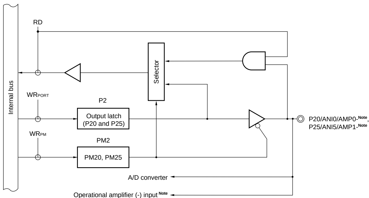
Figure 4-1. Block Diagram of P20 and P25
