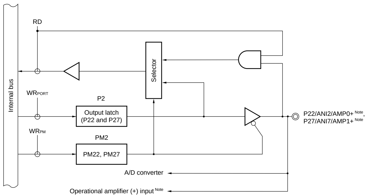
Figure 4-3. Block Diagram of P22 and P27
