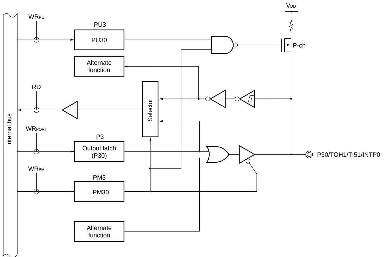
Figure 4-11. Block Diagram of P30
