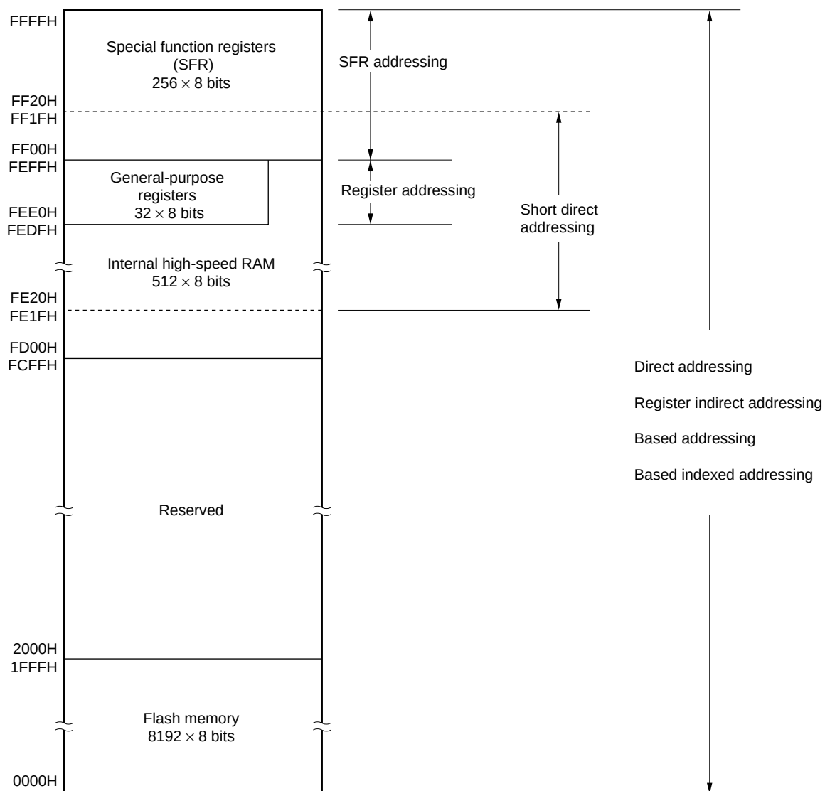
Figure 3-5. Correspondence Between Data Memory and Addressing (R7F0C301x, R7F0C304x, R7F0C307x, R7F0C310x)
