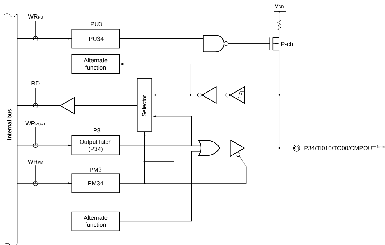
Figure 4-15. Block Diagram of P34
