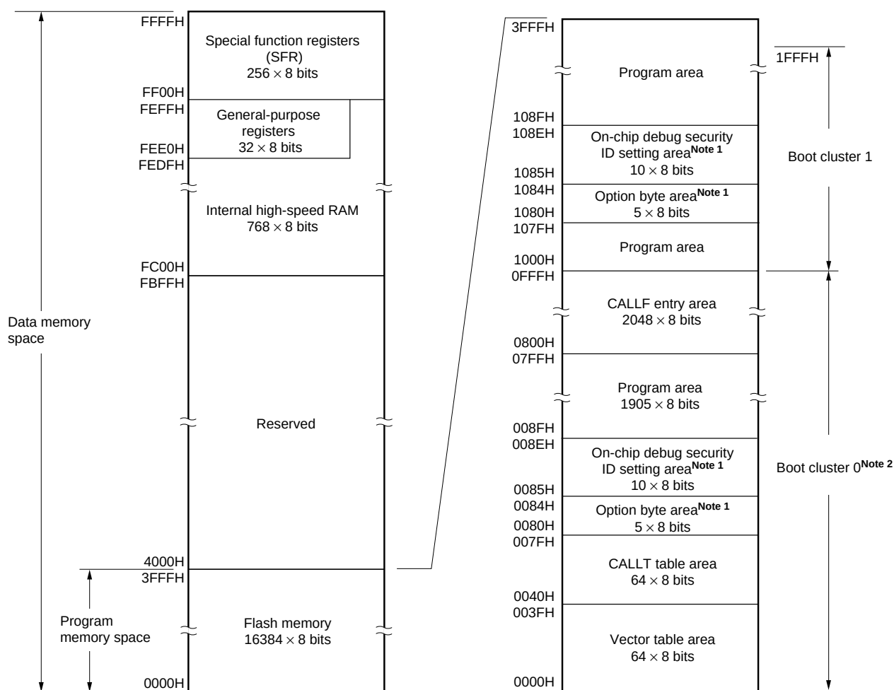
Figure 3-3. Memory Map (R7F0C302x, R7F0C305x, R7F0C308x, R7F0C311x)
