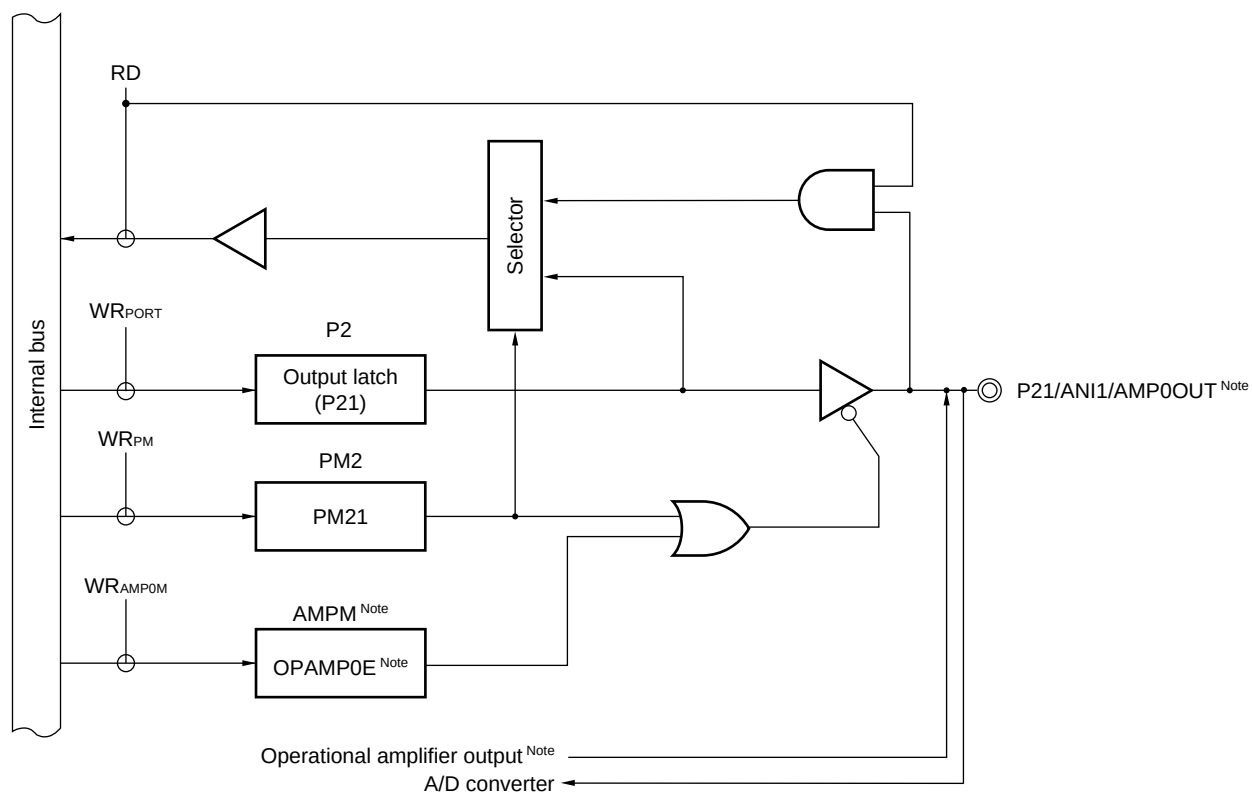
Figure 4-5. Block Diagram of P21
