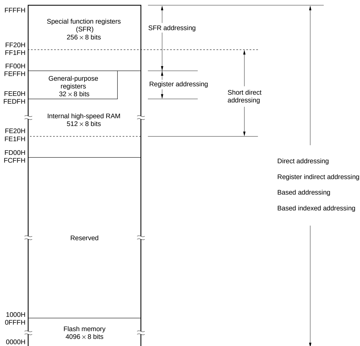
Figure 3-4. Correspondence Between Data Memory and Addressing (R7F0C300x, R7F0C303x, R7F0C306x, R7F0C309x)
