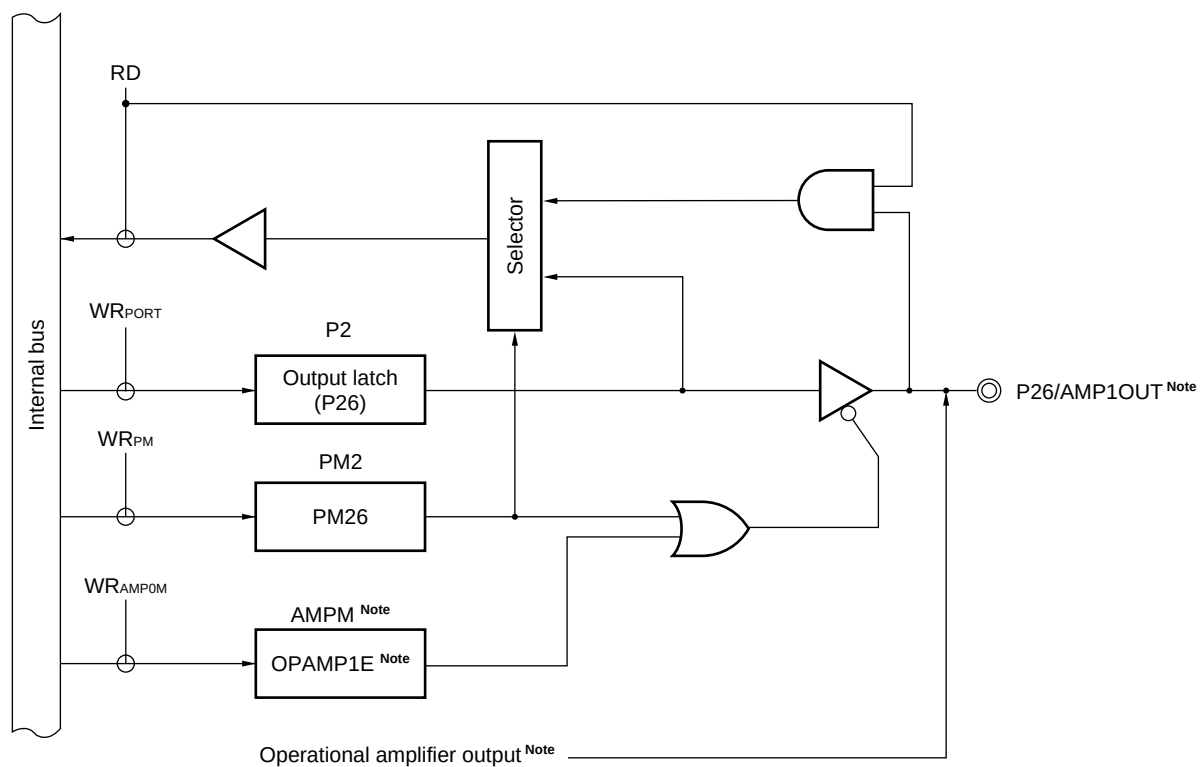
Figure 4-9. Block Diagram of P26
