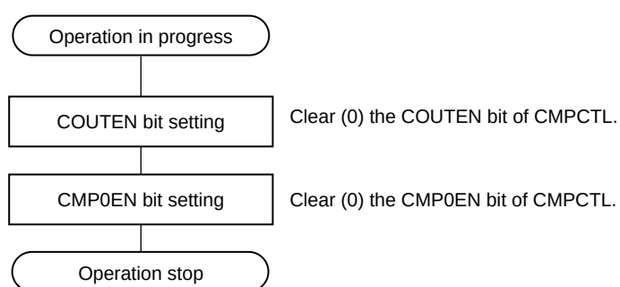
Figure 12-7. Example of Setting Procedure when Stopping Comparator Operation
