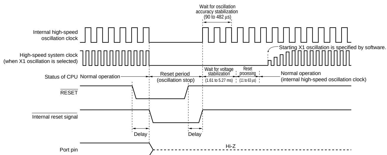
Figure 16-2. Timing of Reset by RESET Input
