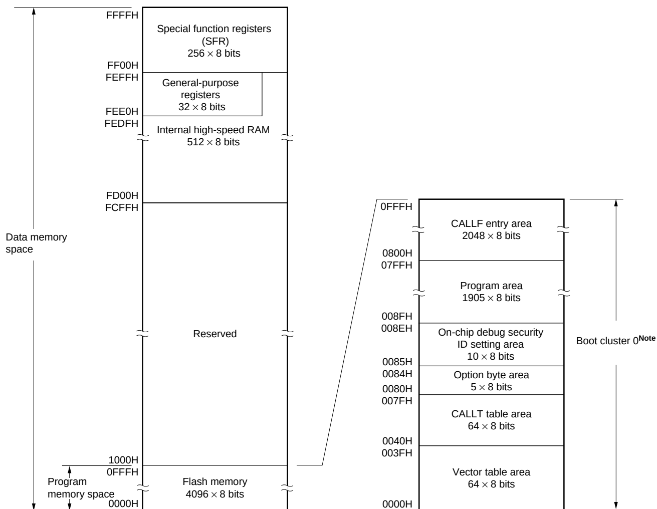
Figure 3-1. Memory Map (R7F0C300x, R7F0C303x, R7F0C306x, R7F0C309x)
