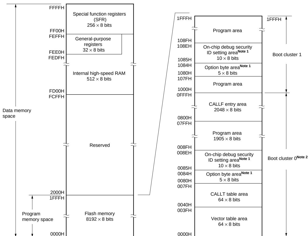
Figure 3-2. Memory Map (R7F0C301x, R7F0C304x, R7F0C307x, R7F0C310x)
