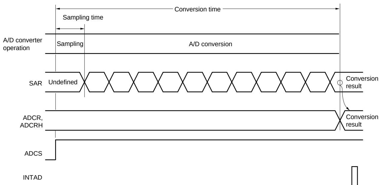
Figure 10-12. Basic Operation of A/D Converter
