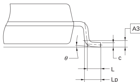
detail of lead end
