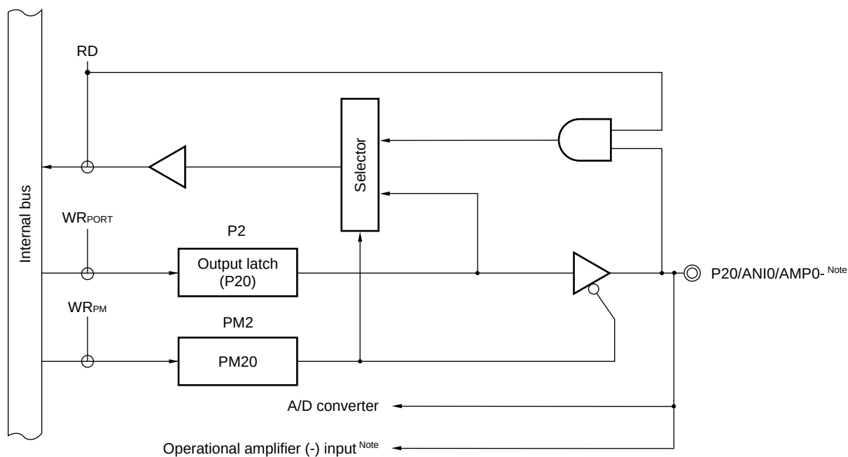
Figure 4-4. Block Diagram of P20
