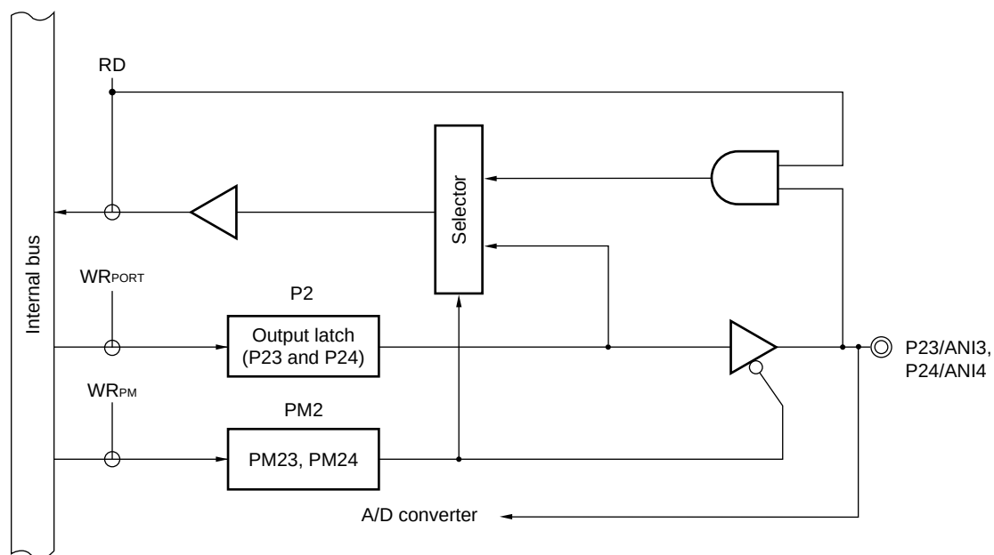
Figure 4-7. Block Diagram of P23, P24
