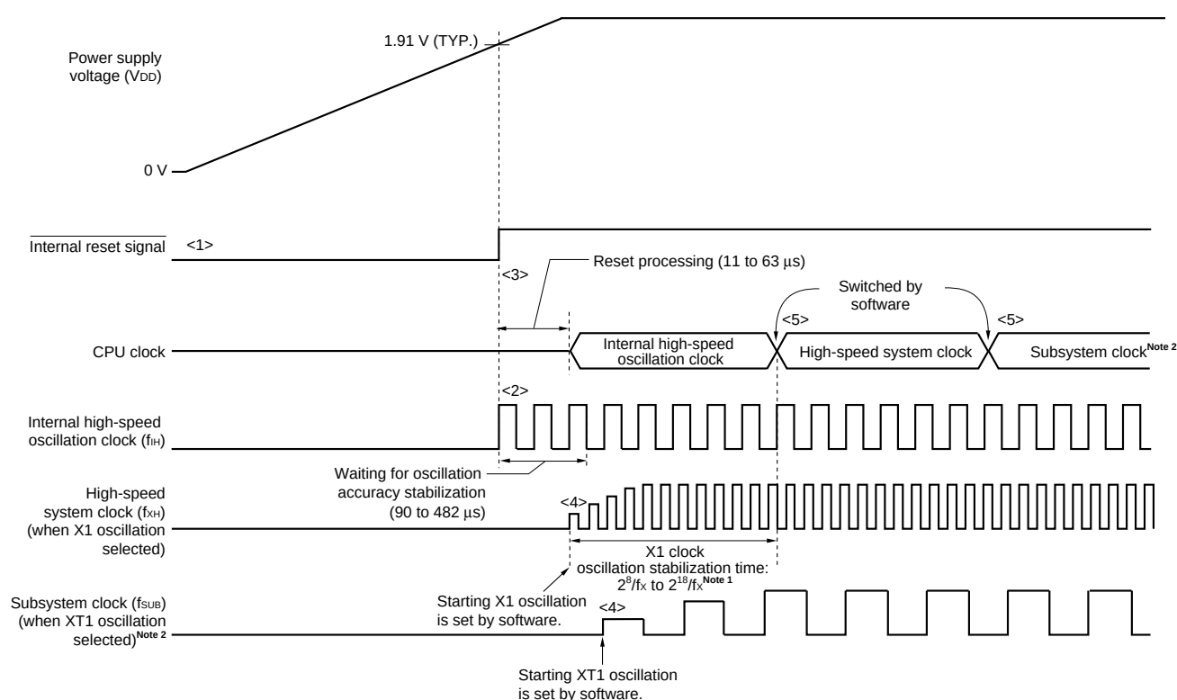
Figure 5-12. Clock Generator Operation When Power Supply Voltage Is Turned On (When LVI Default Start Function Enabled Is Set (Option Byte: LVISTART = 1))
