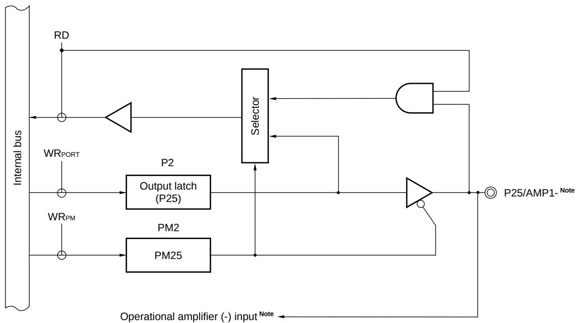
Figure 4-8. Block Diagram of P25
