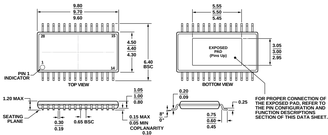
Figure 55. 28-Lead Thin Shrink Small Outline Package, Exposed Pad [TSSOP_EP] (RE-28-2) Dimensions shown in millimeters
