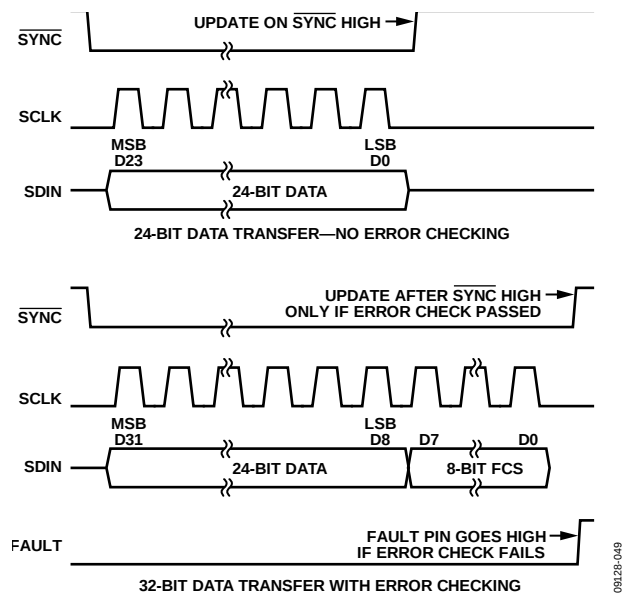
Figure 41. PEC Timing
