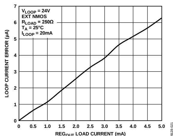
Figure 23. Loop Current Error vs. REG_{OUT} Load Current
