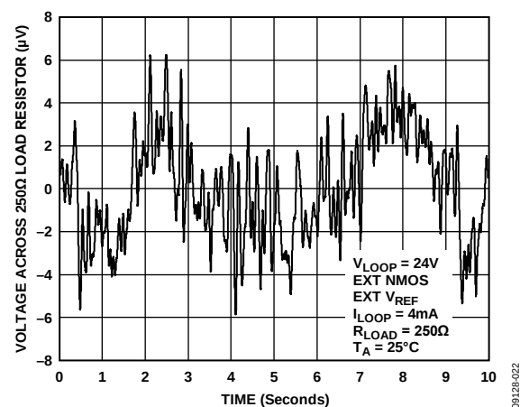
Figure 24. Loop Current Noise, 0.1 Hz to 10 Hz Bandwidth
