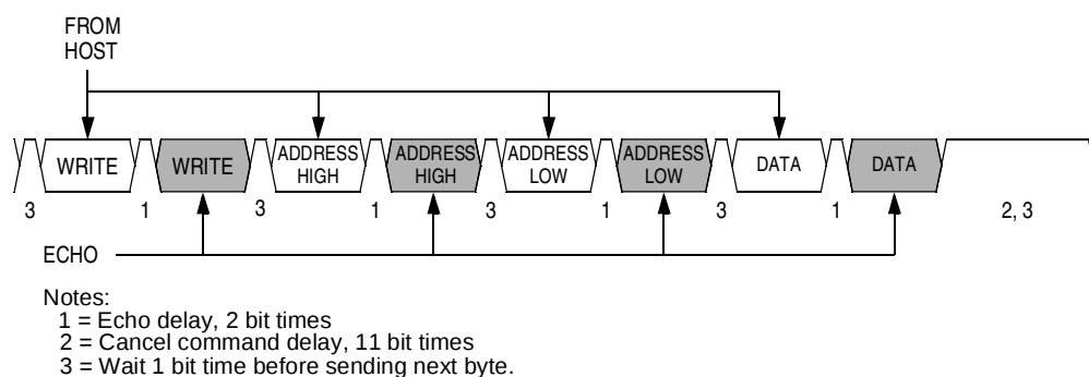
Figure 15-8. Write Transaction
