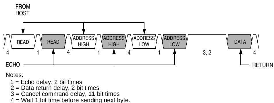
Figure 15-7. Read Transaction
