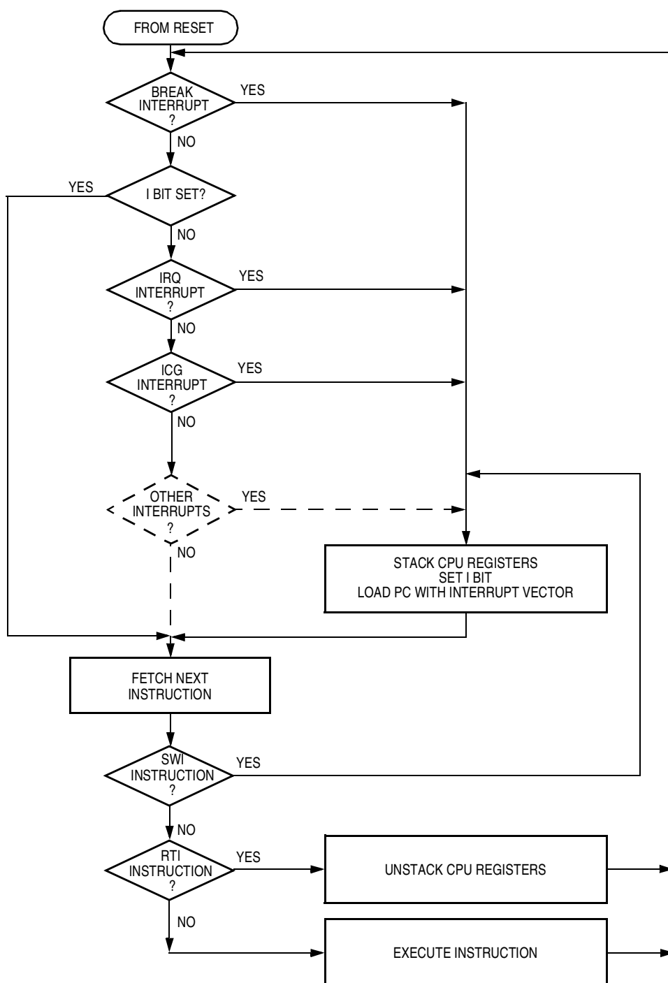
Figure 4-6. Interrupt Processing
