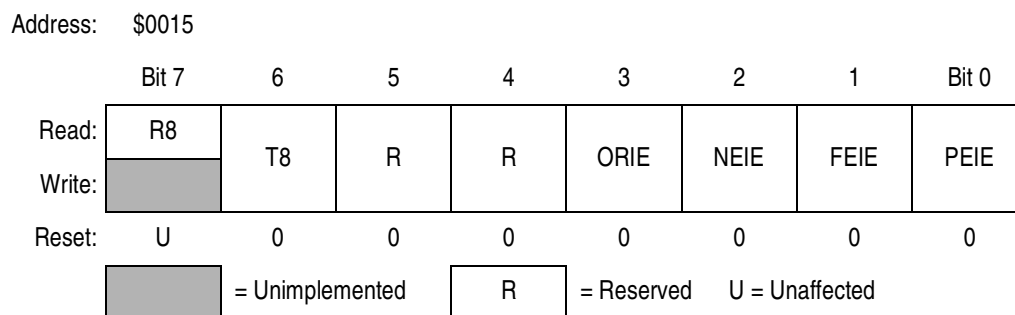
Figure 18-11. ESCI Control Register 3 (SCC3)
