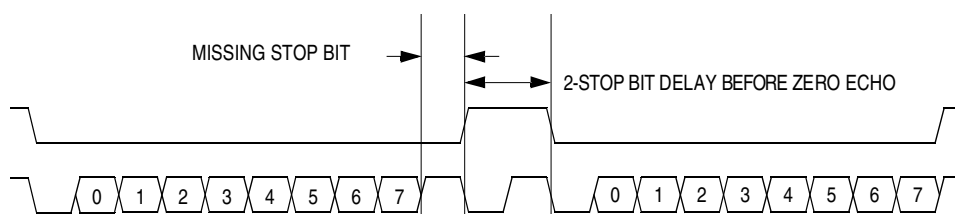
Figure 15-6. Break Transaction
