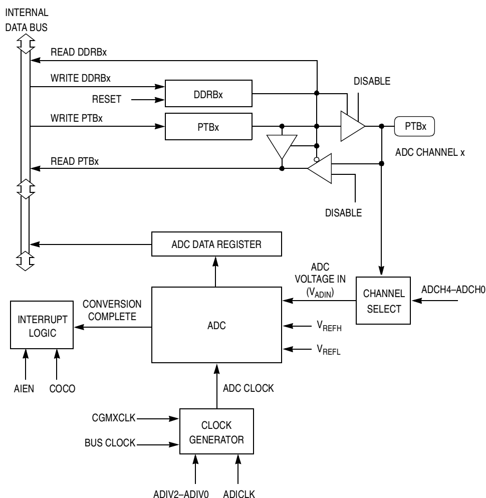
Figure 5-1. ADC Block Diagram
