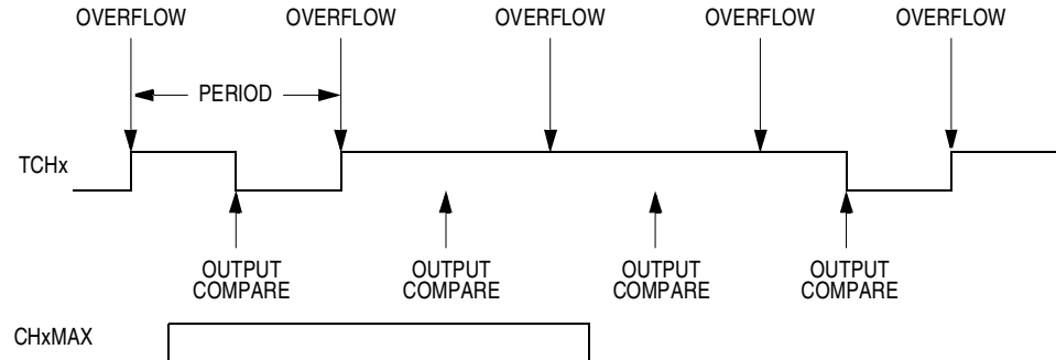
Figure 22-11. CHxMAX Latency
