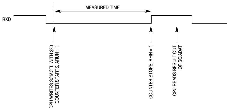
Figure 18-21. Bit Time Measurement with ACLK = 1, Scenario A
