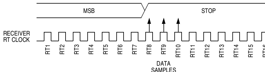
Figure 18-7. Slow Data
