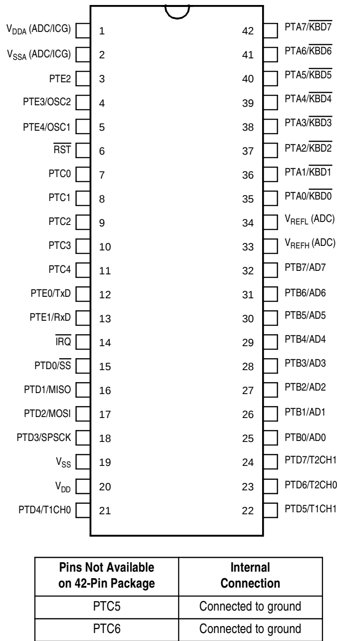
Figure 1-2. 42-Pin SDIP Pin Assignments
