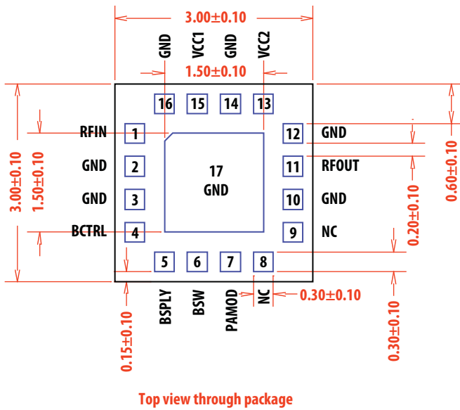
Figure 46. Package dimensions
