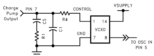
FIGURE 18. VCXO
