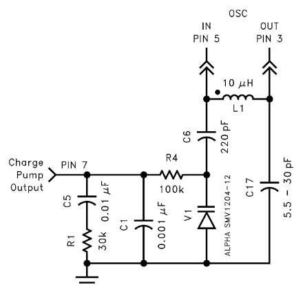
FIGURE 20. LC TANK
