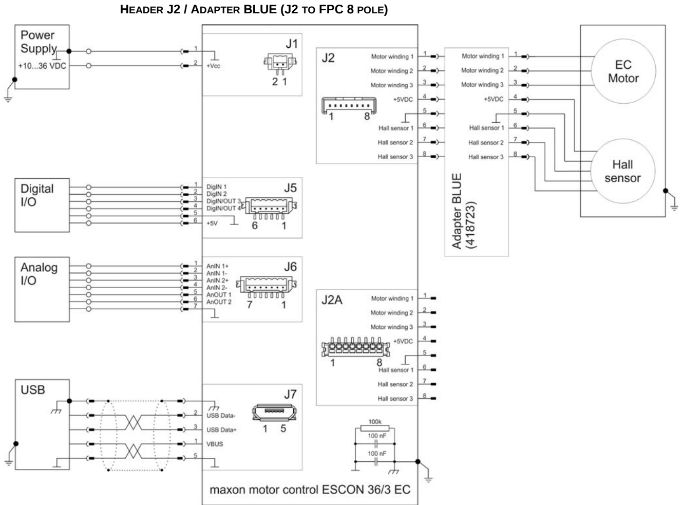
Figure 4-24 maxon EC motor with Hall Sensors (J2 and Adapter BLUE)
