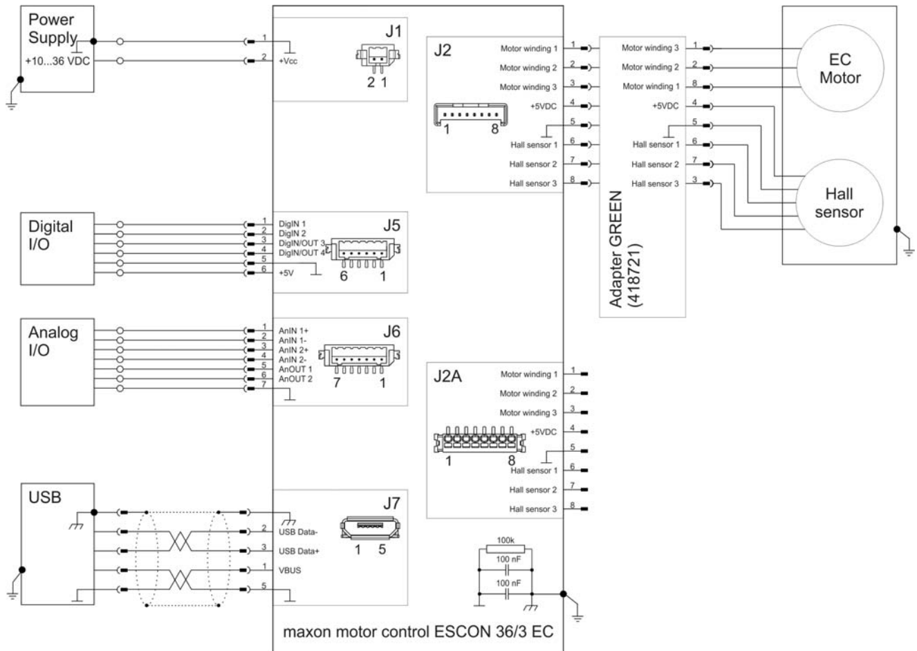
Figure 4-25 maxon EC motor with Hall Sensors (J2 and Adapter GREEN)
