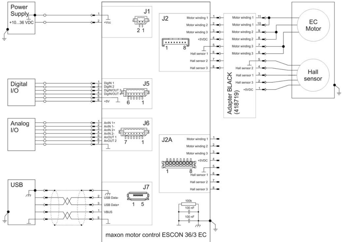
Figure 4-23 maxon EC motor with Hall Sensors (J2 and Adapter BLACK)
