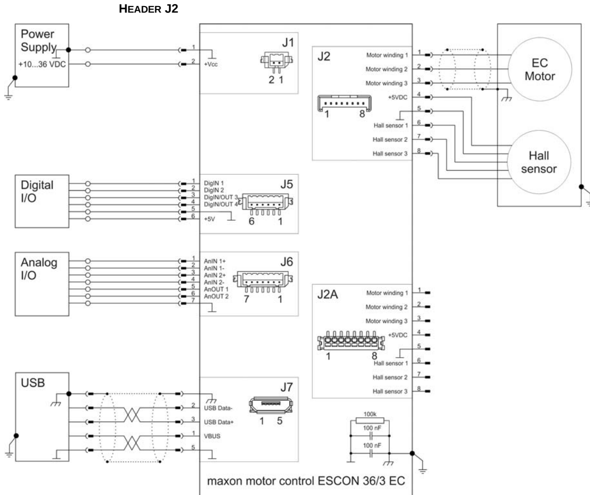
Figure 4-21 maxon EC motor with Hall Sensors (J2)
