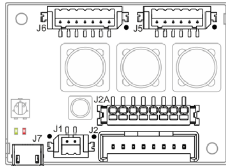
Figure 4-20 Interfaces – Designations and Location
