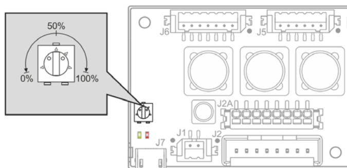
Figure 3-18 Potentiometer P1 – Location & Adjustment Range
