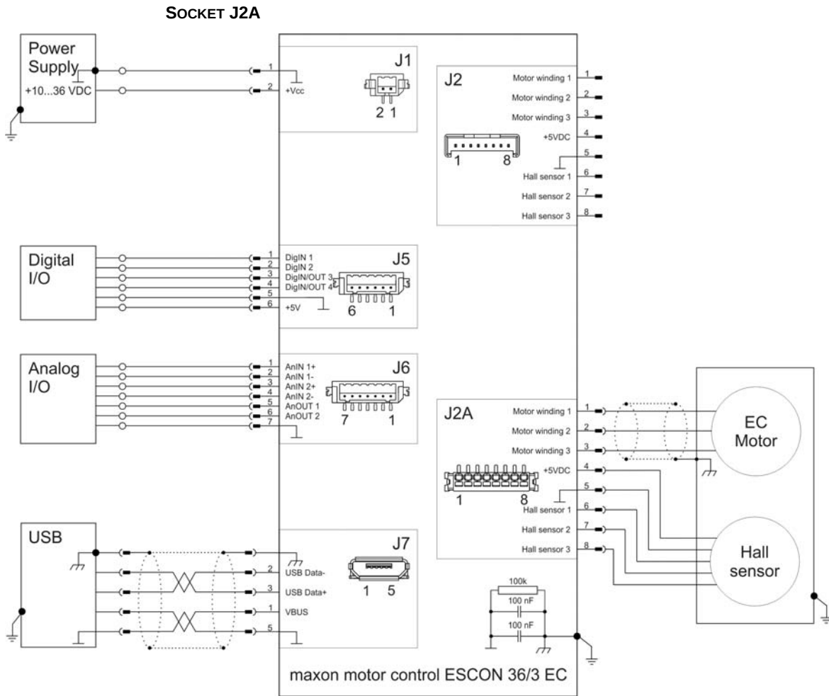
Figure 4-22 maxon EC motor with Hall Sensors (J2A)
