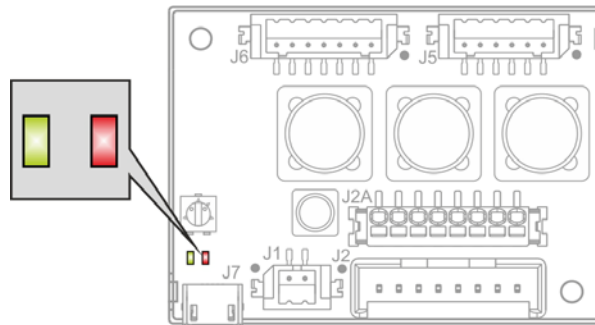
Figure 3-19 LEDs – Location
