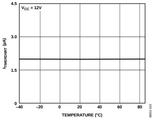
Figure 22. Timer Pull-Down Current, Retry ( I_{\text{TIMERDNRT}} ) vs. Temperature
