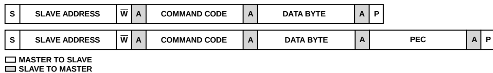
Figure 60. Write Byte and Write Byte with PEC
