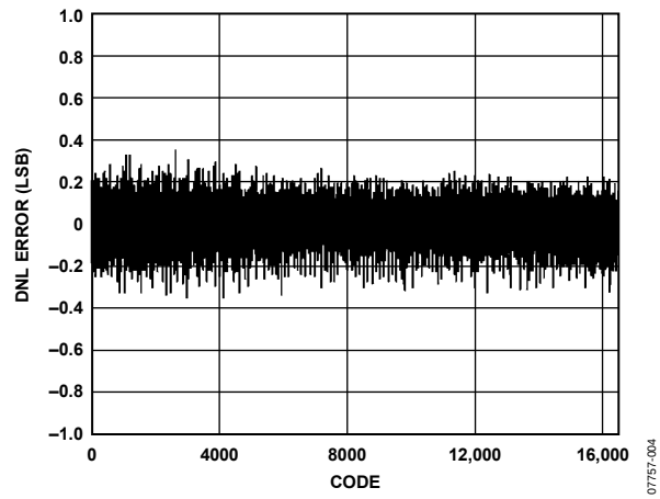
Figure 4. Typical DNL
