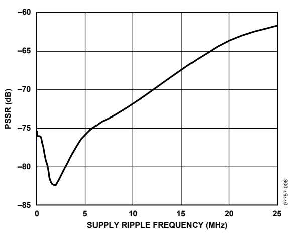
Figure 8. PSRR vs. Supply Ripple with No Supply Decoupling
