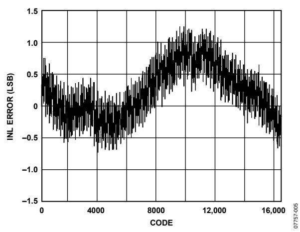
Figure 5. Typical INL
