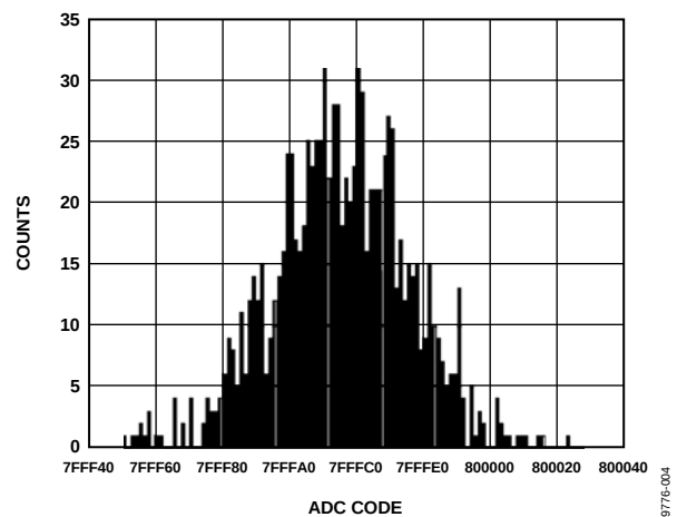
Figure 4. Histogram Showing Output Code Spread with AD7793 Input Pins Shorted Together
