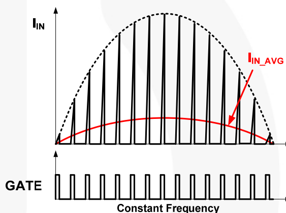
Figure 18. Input Current and Switching
