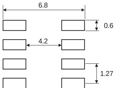
FOOT PRINT DIMENSIONS (in millimeters)
