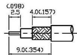
STRIPPING DIMENSION
