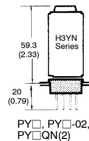
Mounting Height
