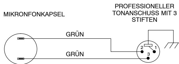
INTERNE ANSCHLÜSSE
