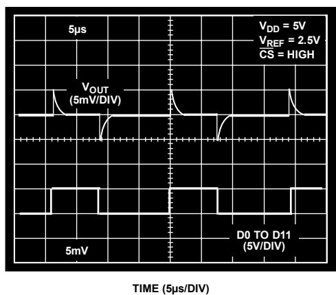
Figure 18. Digital Feedthrough
