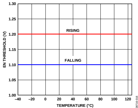
Figure 16. EN Threshold vs. Temperature
