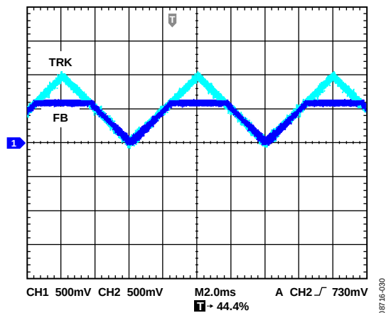
Figure 30. Tracking Function
