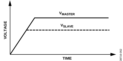
Figure 52. Coincident Tracking
