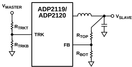
Figure 51. Voltage Tracking
