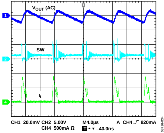
Figure 34. PFM Mode
