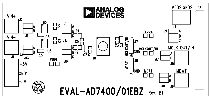
Figure 6. Silkscreen
