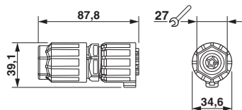
Dimensional drawing: connector, 2.5 mm 2
