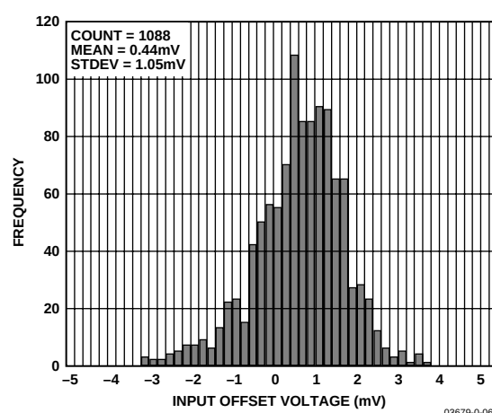
Figure 42. Input Offset Voltage Distribution
