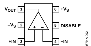
Figure 2. SC70-6 (KS)
