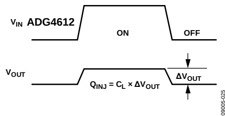
Figure 27. Charge Injection
