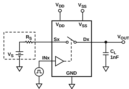
Figure 27. Charge Injection
