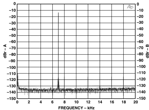
Figure 20. Two-Tone Test
