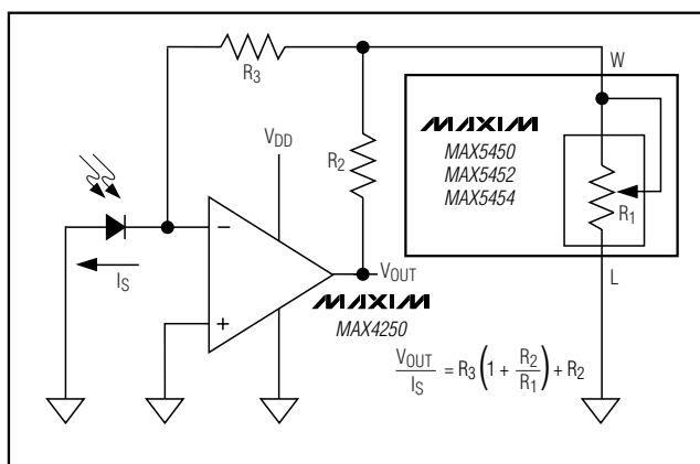
Figure 5. Adjustable Current to Voltage Converter
