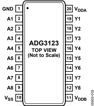
Figure 3. Pin Configuration
