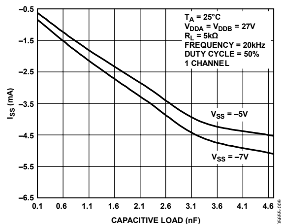
Figure 9. Supply Current ( I_{SS} ) vs. Capacitive Load
