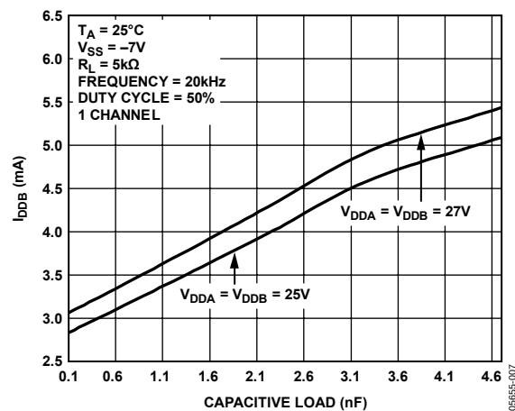
Figure 7. Supply Current ( I_{DDB} ) vs. Capacitive Load
