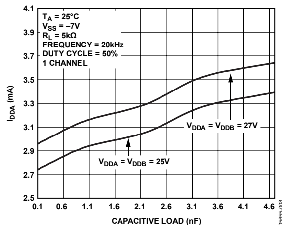
Figure 8. Supply Current ( I_{DDA} ) vs. Capacitive Load
