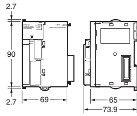
CJ1G-CPU4□P
