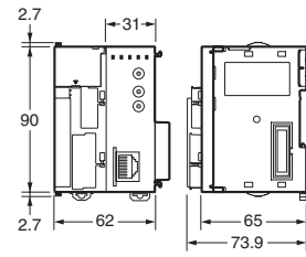
CJ1M-CPU1□-ETN
