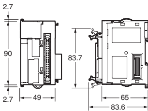
CJ1M-CPU2□
