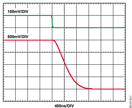
Figure 9. Fall Time
