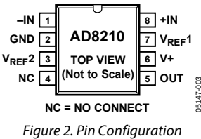
Figure 2. Pin Configuration
