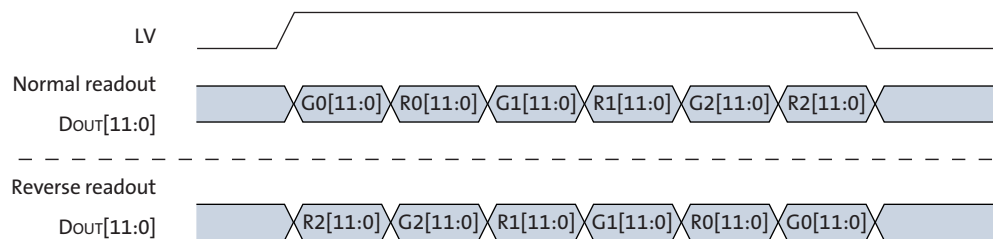
Figure 21: Six Pixels in Normal and Column Mirror Readout Modes
