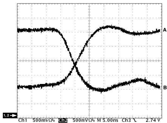
TPC 14. Loaded Driver Differential Outputs
