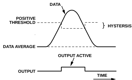
Figure 19. Threshold Hysteresis
