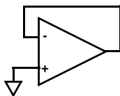
FIGURE 39. PREVENTING OSCILLATIONS IN UNUSED CHANNELS
