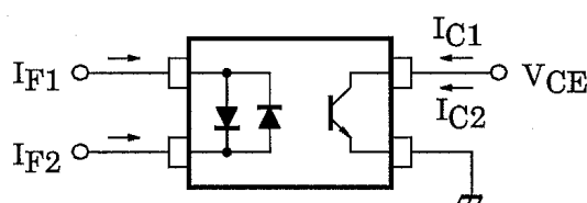
Fig. 8.1 Collector Current Ratio Test Circuit
