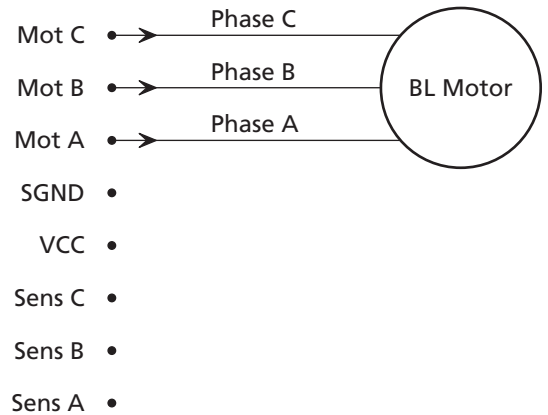
BL motor without hall sensors (not SC5004/SC5008)
