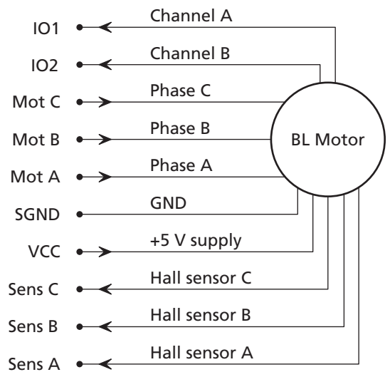
BL motor with digital hall sensors and encoder IE 2 (not SC1801)
