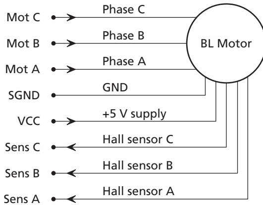
BL motor with digital/analog hall sensors
