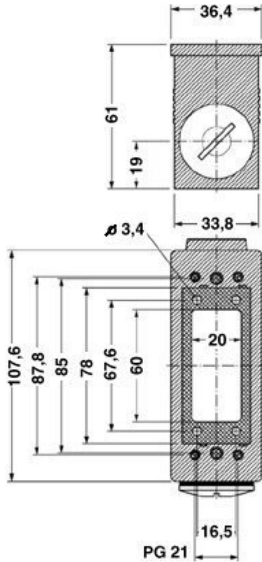
Dimensioned drawing
