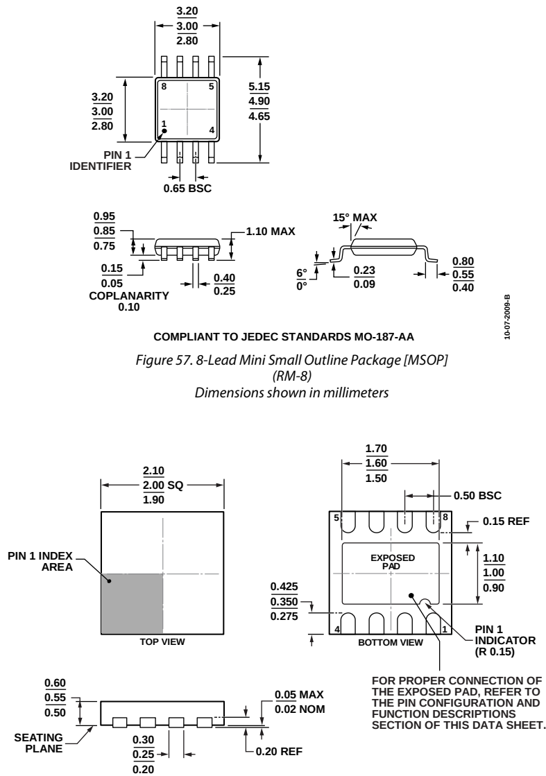
Figure 58. 8-Lead Lead Frame Chip Scale Package [LFCSF_UD] 2 mm x 2 mm Body, Ultra Thin, Dual Lead (CP-8-10) Dimensions shown in millimeters
