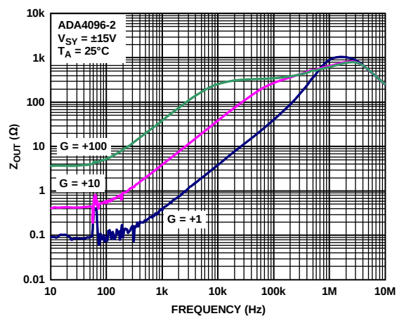
Figure 41. Output Impedance vs. Frequency
