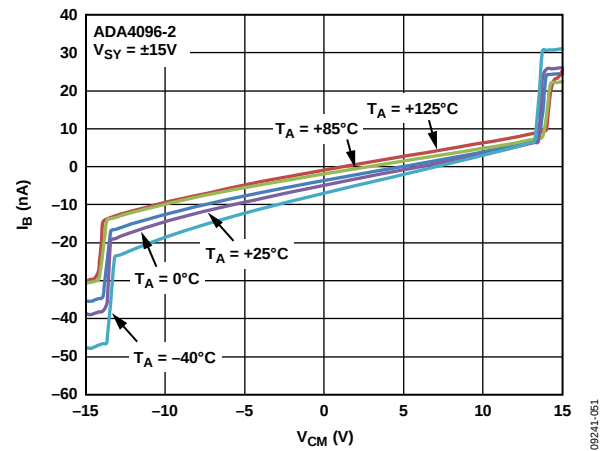
Figure 37. Input Bias Current vs. V_{CM} and Temperature
