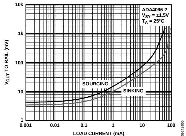
Figure 12. Dropout Voltage vs. Load Current
