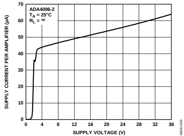
Figure 50. Supply Current vs. Supply Voltage
