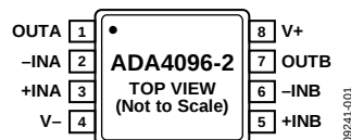
Figure 1. 8-Lead, MSOP (RM-8), ADA4096-2
