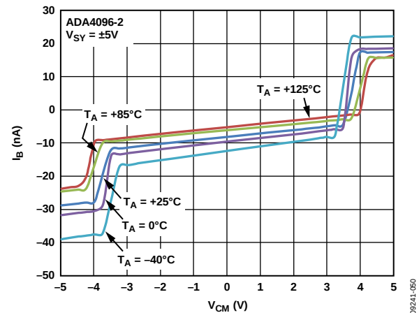
Figure 24. Input Bias Current vs. V_{CM} and Temperature
