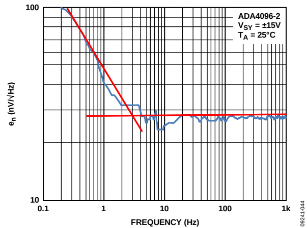
Figure 51. Voltage Noise Density
