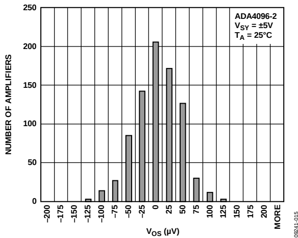
Figure 21. Input Offset Voltage Distribution
