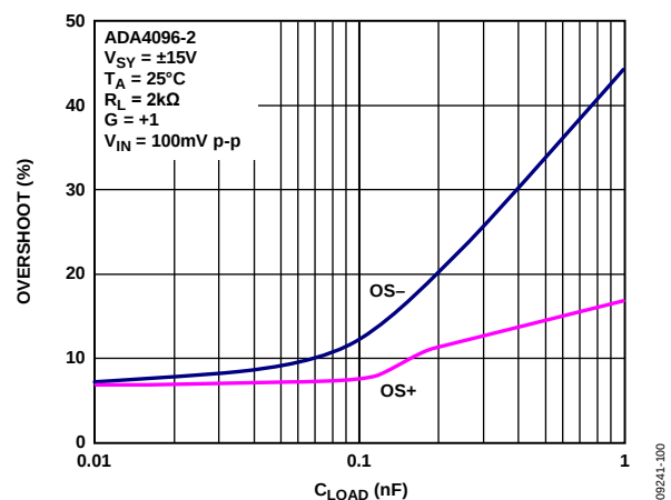
Figure 52. Overshoot vs. Load Capacitance
