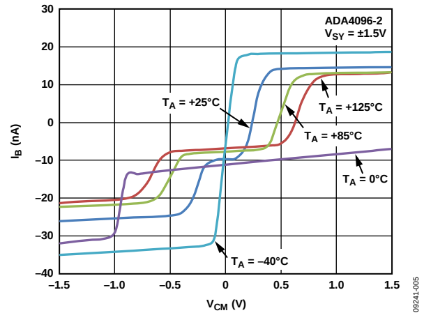
Figure 11. Input Bias Current vs. V_{CM} and Temperature
