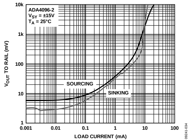
Figure 38. Dropout Voltage vs. Load Current
