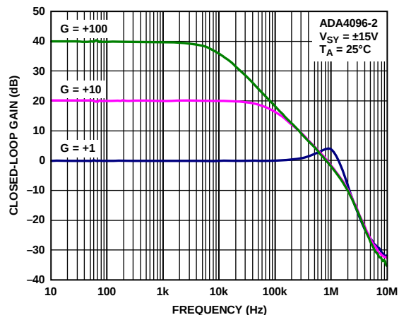
Figure 40. Closed-Loop Gain vs. Frequency
