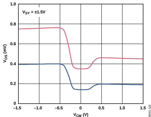
Figure 10. CMRR Sweep, \pm 3\text{ V}
