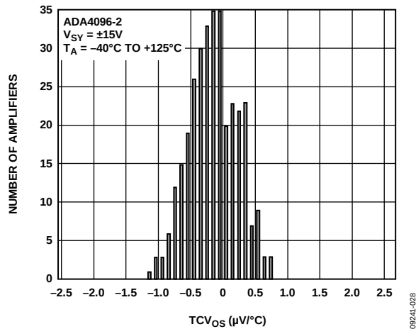
Figure 35. Offset Voltage Drift Distribution
