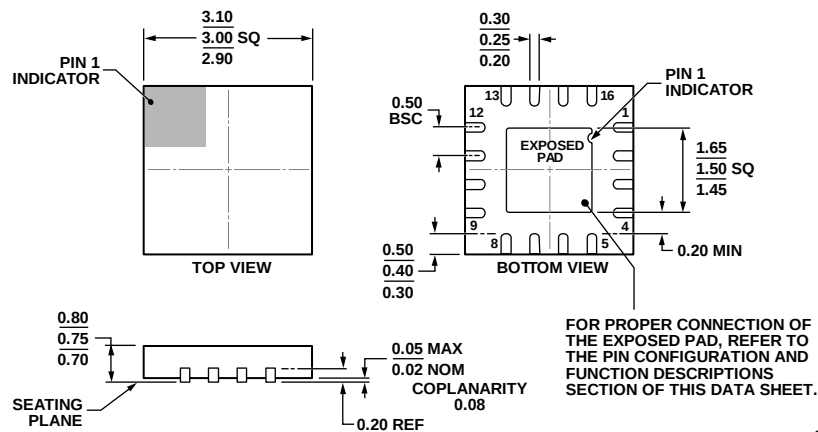
Figure 60. 16-Lead Lead Frame Chip Scale Package [LFCSP_WQ] 3 mm × 3 mm Body, Very Very Thin Quad (CP-16-27)
