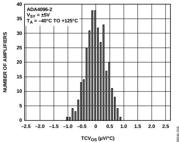
Figure 22. Offset Voltage Drift Distribution
