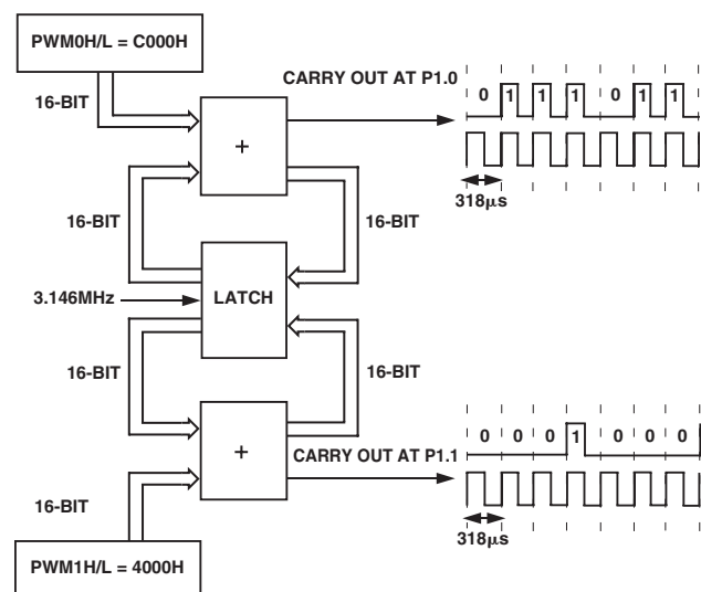
Figure 32. PWM Mode 6
