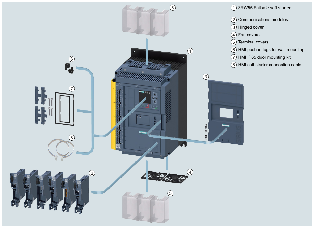
SIRIUS 3RW55 Failsafe High Performance soft starter with accessories (see page 6/53)
