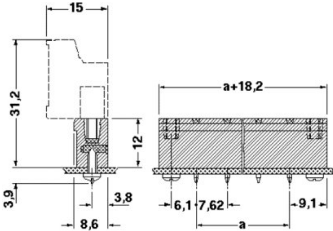
Dimensioned drawing
