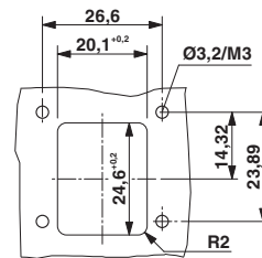
Dimensioned drawing
