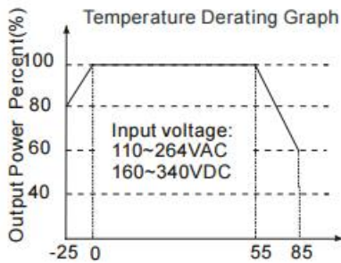
Temperature vs load
