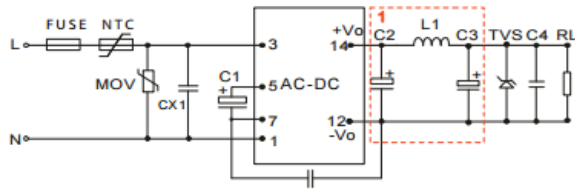
Figure 1 LS05-15BXXS
