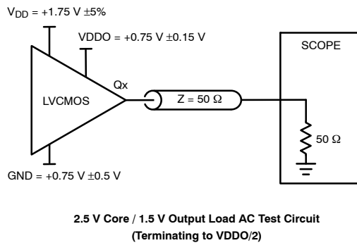
Figure 3. Operational Supply and Termination Test Conditions
