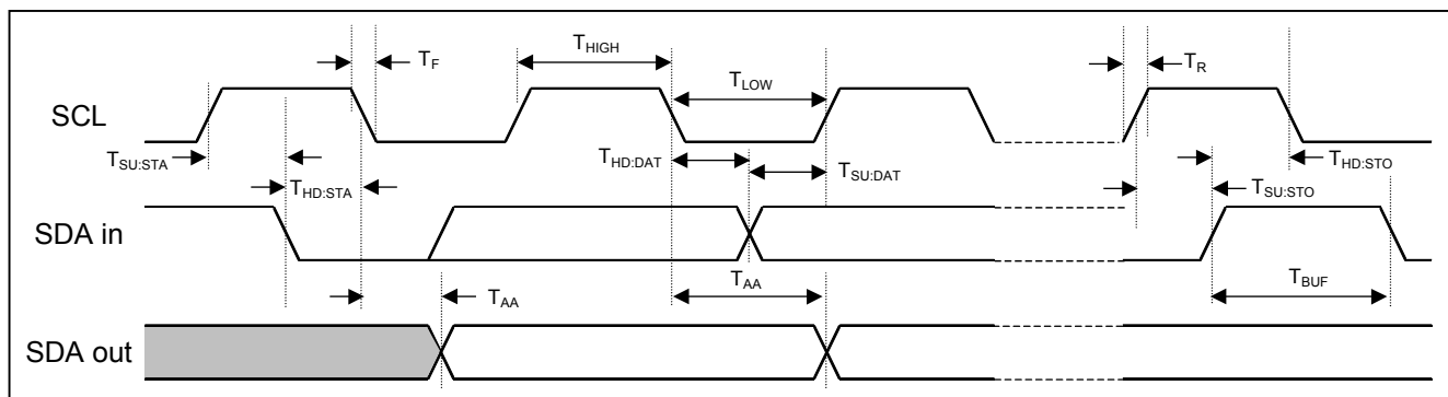
FIG. 7 - I 2 C Bus Data Requirements
