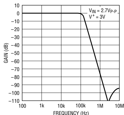
Frequency Response
