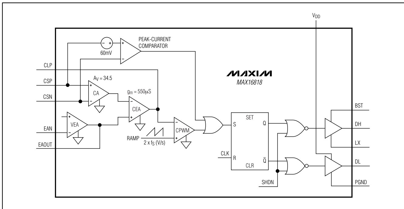
Figure 8. MAX16818 Phase Circuit
