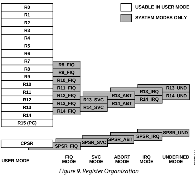
Figure 9. Register Organization
