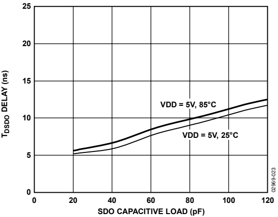
Figure 23. t_{\text{SDO}} Delay vs. Capacitance Load and Supply
