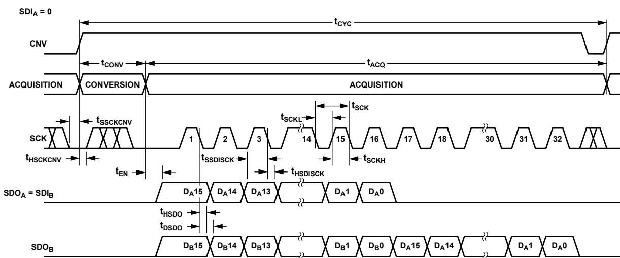
Figure 42. Chain Mode, No Busy Indicator Serial Interface Timing
