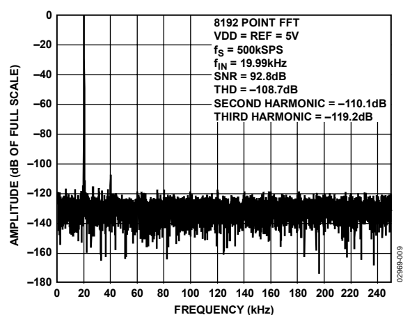
Figure 9. FFT Plot
