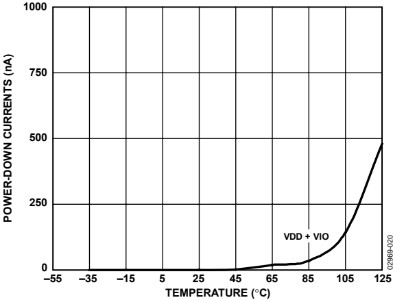
Figure 20. Power-Down Currents vs. Temperature
