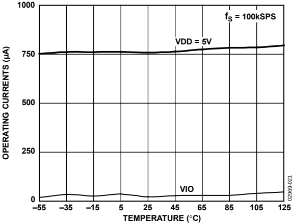
Figure 21. Operating Currents vs. Temperature
