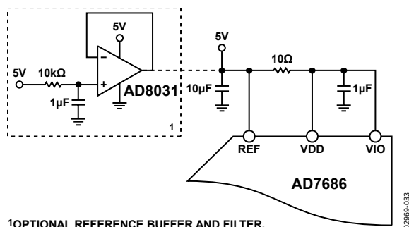
Figure 32. Example of Application Circuit
