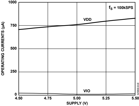
Figure 19. Operating Currents vs. Supply
