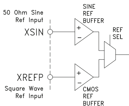
Figure 1. Reference Sine Input Stages
