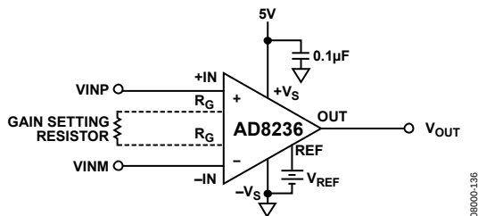
Figure 35. Basic Setup
