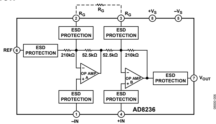
Figure 34. Simplified Schematic
