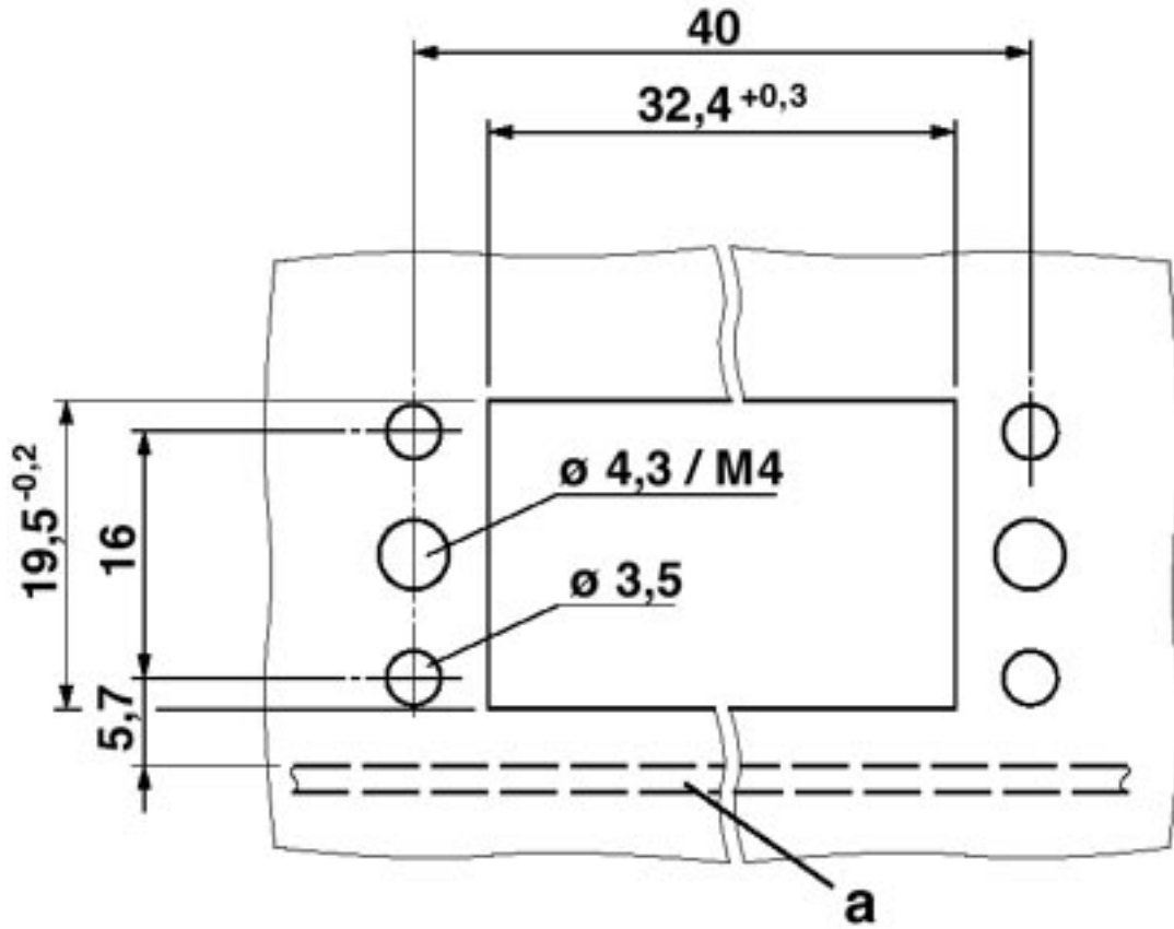
Dimensioned drawing
